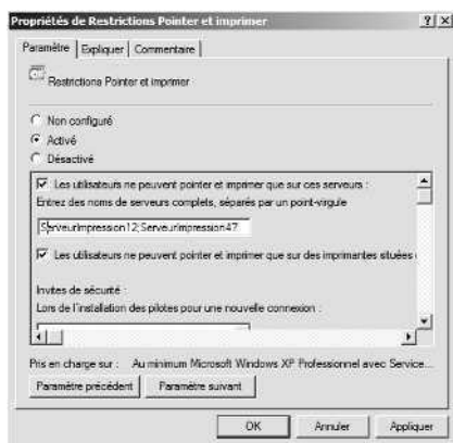
Figure 18-7 Configurez les Restrictions Pointer et imprimer.
